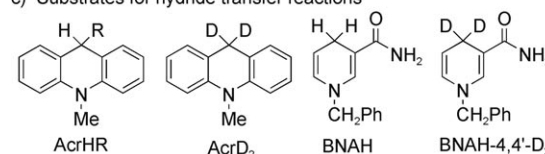
Scheme 1. Iron(IV)–oxo porphyrins and substrates used in this study.
